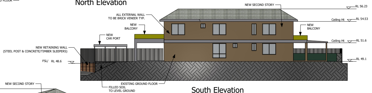
North Elevation
